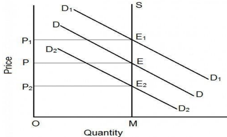
Fig.1.1 Perishable Goods
