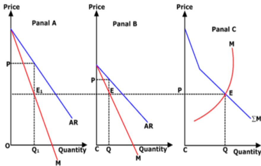
Fig. 2.4. Price Discrimination
